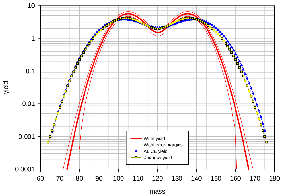
Benchmark B: ^{241}\text{Am} at 28 MeV, pre-neutron emission mass distribution
